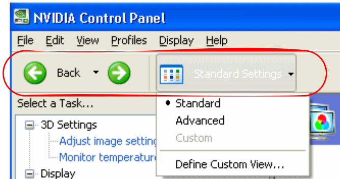
Figure 3.4 Toolbar
